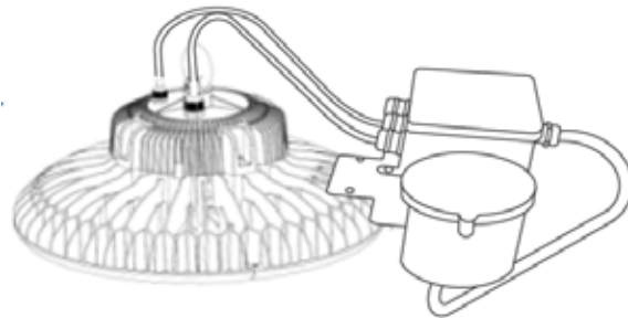
Waterproof Junction Box, Bracket Mount and Sensor options available
